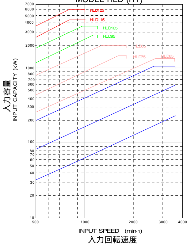
ポンプ用 CAPACITY CHART OMEGA CLUTCH FOR PUMP MODEL HLD (HY)
